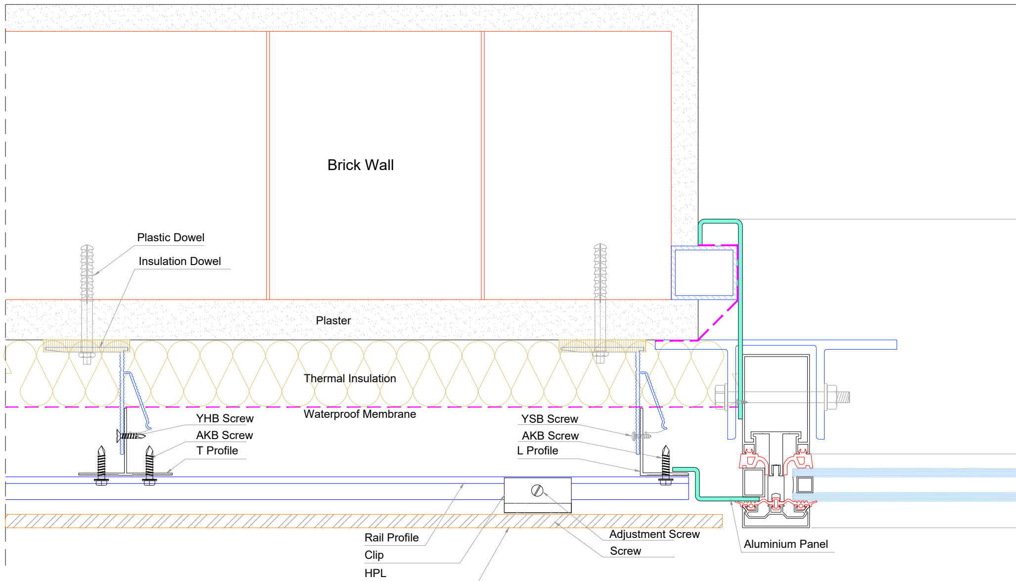
DETAIL A
